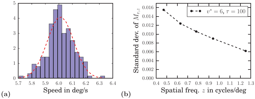
Figure 7: Simulation of the speed distributions of a set of motion clouds with the experimentally tested parameters. (a) Histogram of estimates of \hat{v}^{MLE}(I_{v,z}) for z = 0.8 c/° defined by equation 4.8. These estimates are well approximated by a gaussian distribution (red dashed line). (b) Standard deviation of estimates of \hat{v}^{MLE}(I_{v,z}) as a function of z . The standard deviation of these estimates is inversely proportional to the spatial frequency z .
