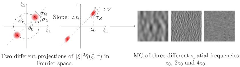
Figure 2: Graphical representation of the covariance \hat{\gamma} shown as a projection on the spatial frequency plane (left) and the spatiotemporal frequency plane (middle). Note the cone-like shape of the envelopes in both cases. The three luminance stimulus images on the right are an example of synthesized frames for three different spatial frequencies, respectively, from left to right, a low, a medium, and a high frequency.
